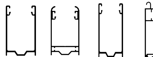
Coulisse alu 40x27 Coulisse alu 45x27 Coulisse alu 50x27 Lame finale alu 14mm
