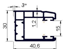
Coulisse PVC 40x30
