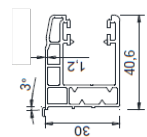
Coulisse PVC 40x30
